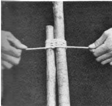
ONE LASHING COMPLETE
