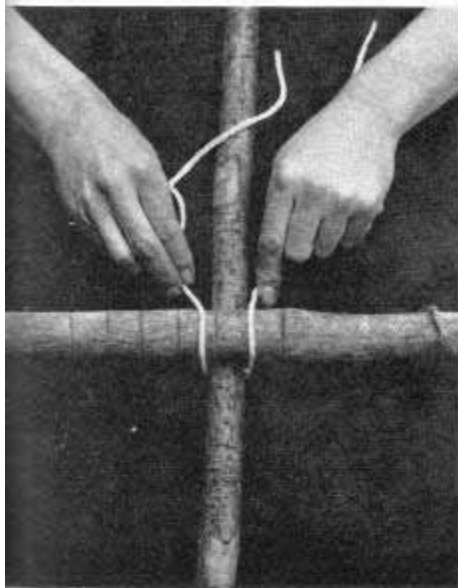
HOW TO BEGIN
