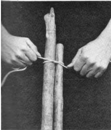
THE FIRST HALF KNOT
